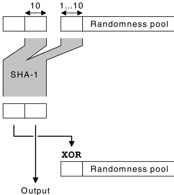
Figure 6.16. The SSLeay/OpenSSL generator's state update and PRNG function.
