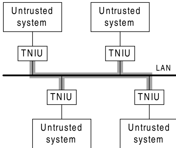
Figure 2.5. Separation kernel implemented using interconnected workstations.
