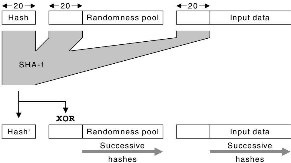
Figure 6.15. The SSLeay/OpenSSL generator's mixing function.
